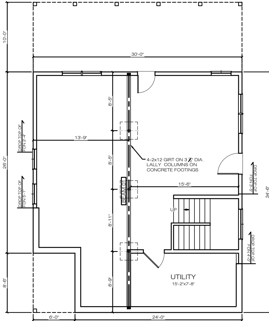
PROP. FOUNDATION PLAN SQ FT: 848
