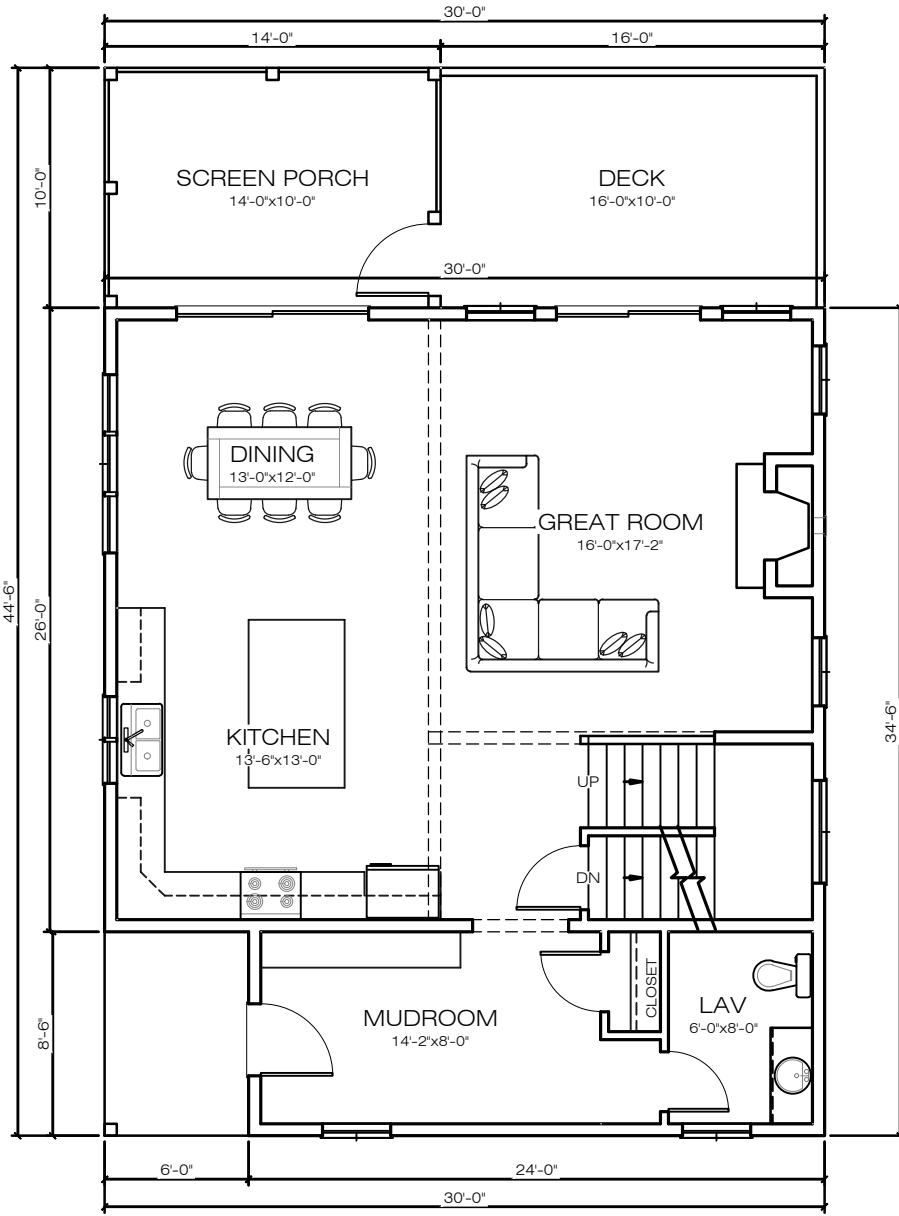
PROP. FIRST FLOOR PLAN SQ FT: 984 CEILING HT: 9' 1-1/8"
